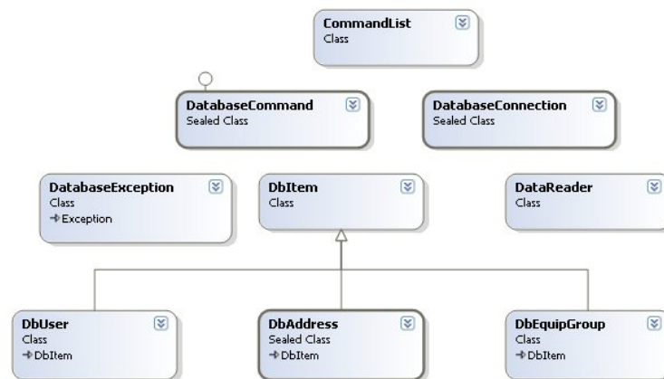
Figure 2.8 - Database Classes
