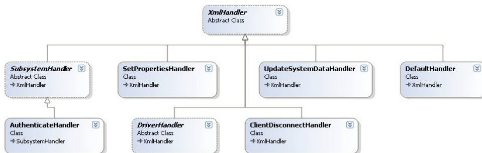
Figure 2.5 - Generic Handlers
